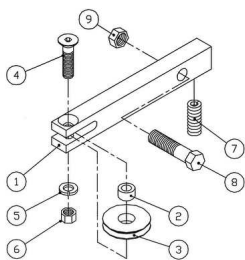
WIRE GUIDE ASSEMBLY
